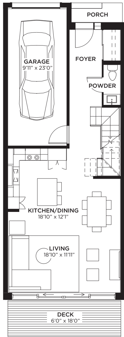
FIRST LEVEL
