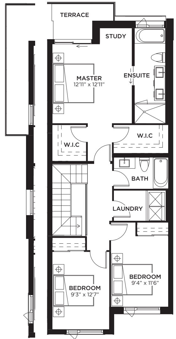
SECOND LEVEL
