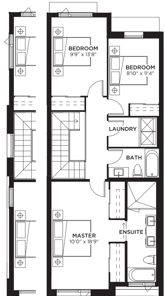
END UNIT
