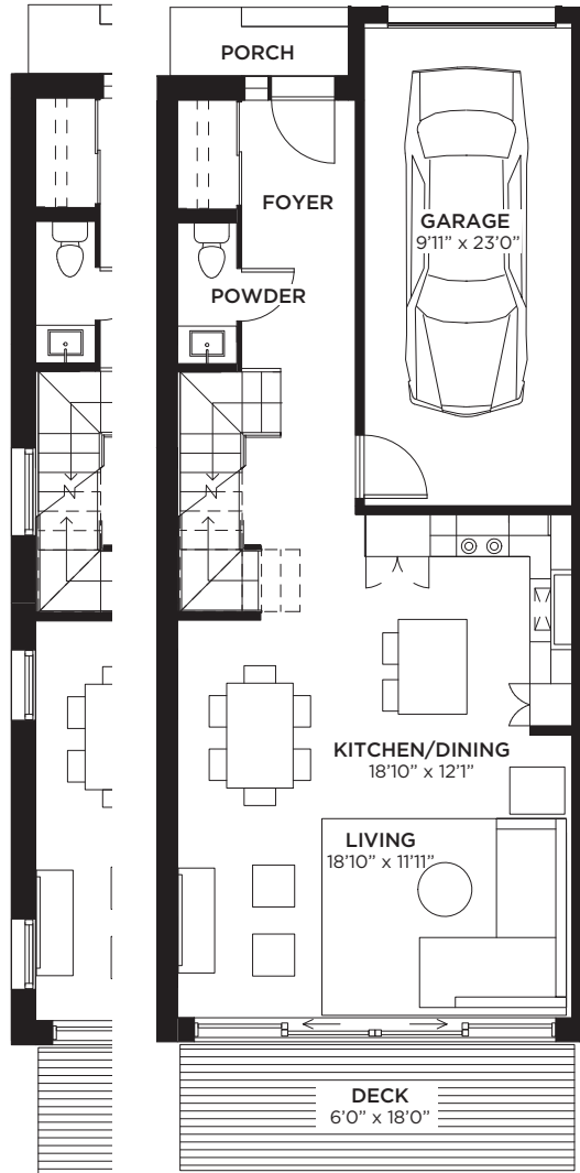
END UNIT
