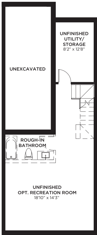
BASEMENT
